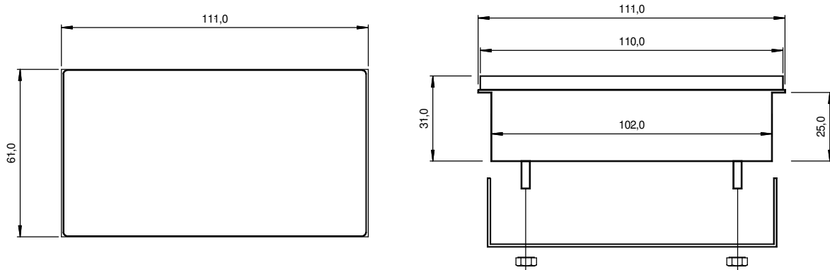
Figure 2: EFI737PRO panel dimensions (mm)
